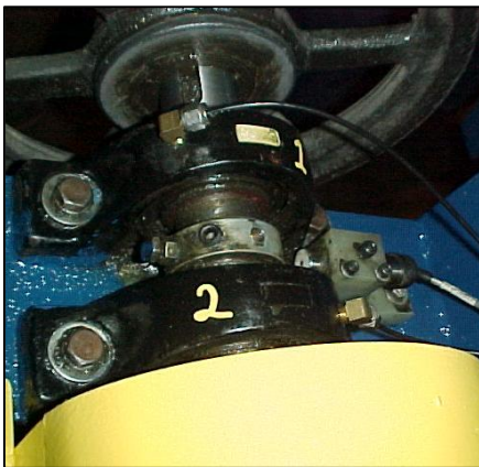
Weekly Operator Lubrication - 8 Lube Points for the Wire Draw machine
